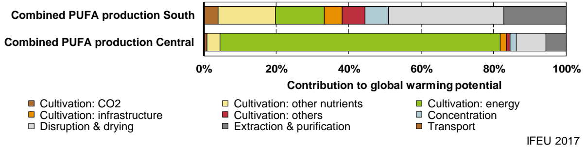
Fig. 4-8 Contributions of processes or inputs to greenhouse gas emissions in Southern and Central Europe (Both scenarios: combined PUFA production with Prorocentrum under optimistic conditions with 80% PV).
