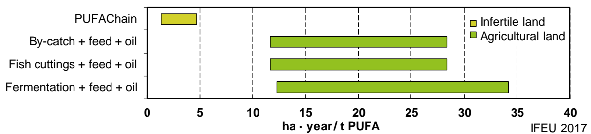
Fig. 4-15 Ranges of land use for all analysed PUFACHain scenarios and all reference systems. Here, PUFACHain scenarios without credits for co-products are compared to a basket of commodities including main and co-products.
