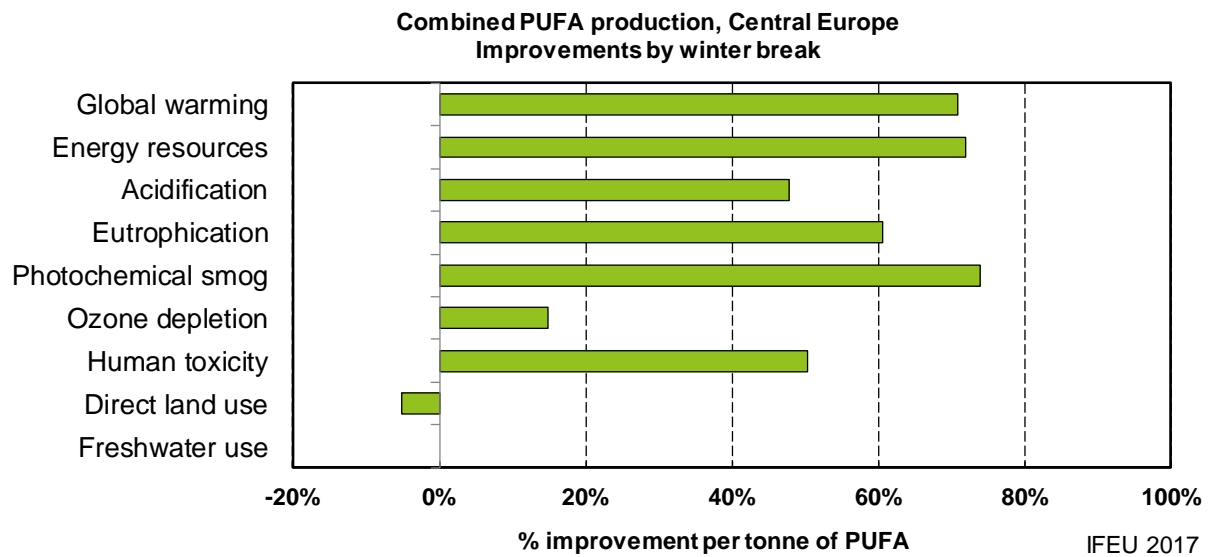
Fig. 4-9 Sensitivity analysis: Reduction/increase of environmental impacts by introducing a three months winter break (Both scenarios: combined PUFA production with Prorocentrum under optimistic conditions with 80% PV in Central Europe).
